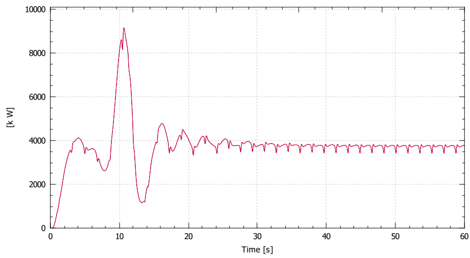
Torque (aero)
